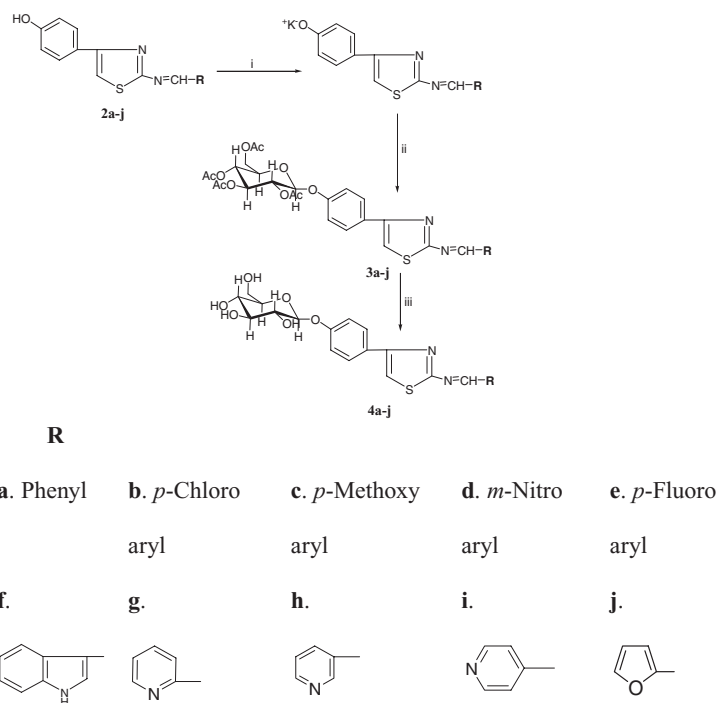
Scheme 2: Synthetic of 2-(substituted benzylideneamino)-4-(4'- o - \beta -D-glucosidoxyphenyl)thiazoles: (i) CH 3 OH, KOH; (ii) acetone, \alpha -acetobromoglucose; (iii) CH 3 ONa, CH 3 OH.
